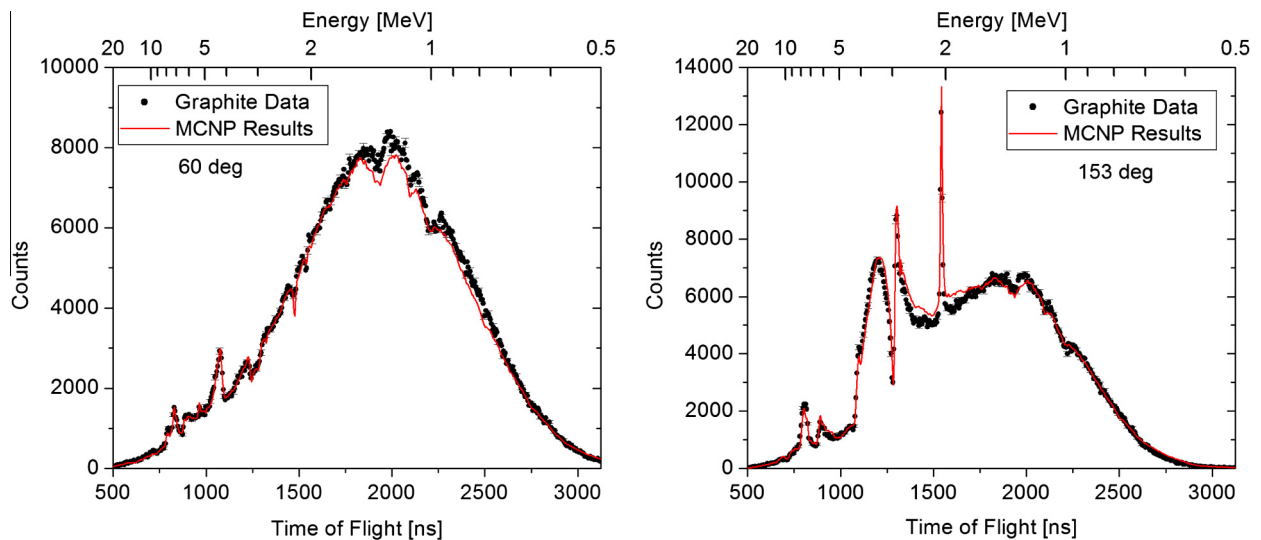
Fig. 6. Detectors 2 (left) and 3 (right) located at 60^\circ and 153^\circ , respectively, with respect to the incident neutron beam. The experimental data collected was part of the second set of angles.
