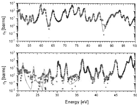
Fig. 5. The measured (scattered points) and fitted ^{247}\text{Cm} (smooth line) fission cross section in the high energy range.
