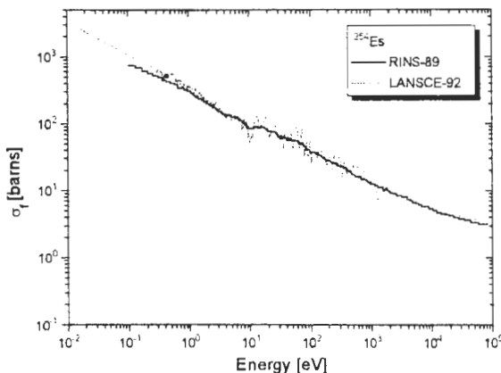
Fig. 2. The ^{254}\text{Es} fission cross section as measured at RINS (solid line) and as measured in LANSCE (dotted line).
