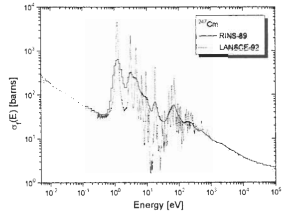
Fig. 3. Fission cross section of ^{247}\text{Cm} as measured at RINS (solid line) and at the LANSCE 1992 experiment (dotted line).
