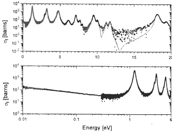
Fig. 4. The measured (scattered points) and fitted ^{247}\text{Cm} (smooth line) fission cross section in the low energy range.
