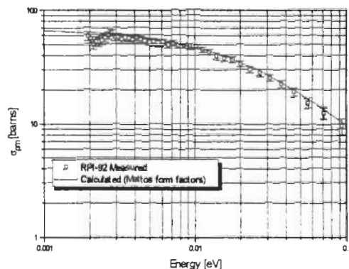
Fig. 8. Ho measured and calculated paramagnetic scattering.
